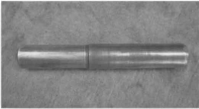
Bushing removal and installation tool. The tool can be used for removal and installation of bushings in both the bell housing and the two pedals
