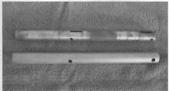
Clutch release shafts. The shaft at the top of the photo is the early type using woodruff keys to lock the lever arm and yoke into place and using 3/16" locking pins. Note the wear on the left end of the shaft and about an inch in from the right end. The shaft at the bottom of the photo is the later type, using 5/16" locking pins. This shaft has only a slight amount of wear on it.
