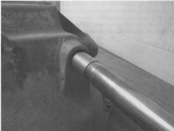
The bushing tool can be used to drive the old bushings out and to drive the new bushings into place.
