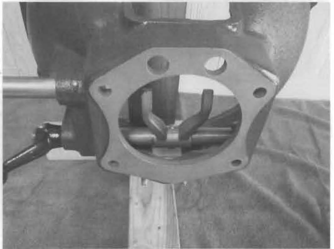
New pedal and clutch release shafts installed. Note operating lever points to the rear when the yoke is standing vertical.
