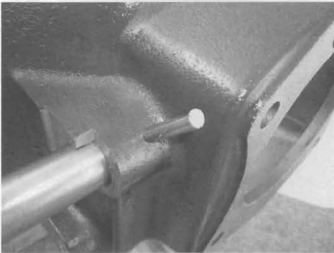
A tapered pin is driven into the bell housing hole to lock the pedal shaft in place.
