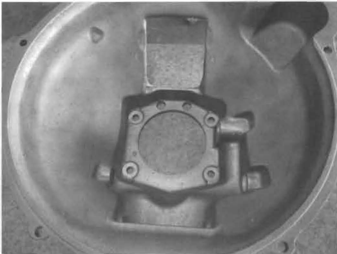
The inside of the bell housing after it was de-greased and bead blasted.
