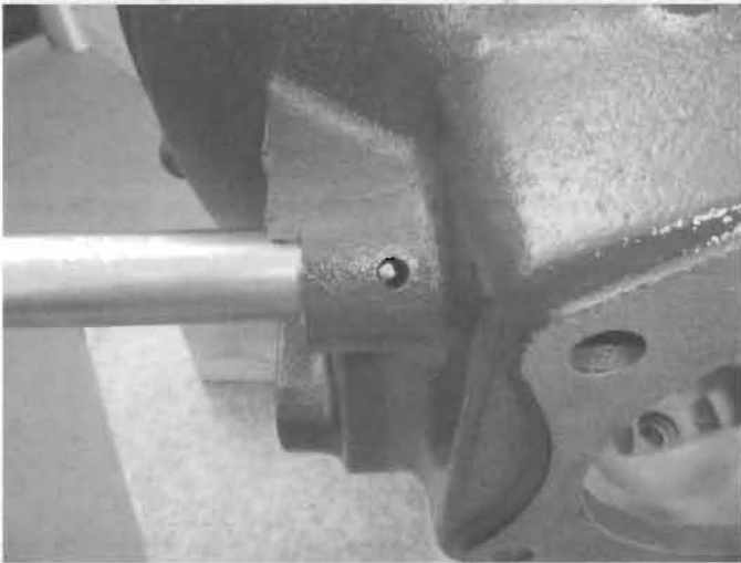
Drive the pedal shaft in until the two holes line up.
