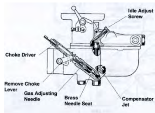
Cut away view of the Model A Carburetor
